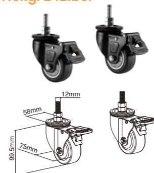
LVS02-CASTER 3" Mobile Caster
