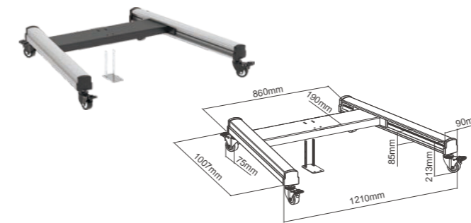
LVS02-B04 H Style Base with Caster
