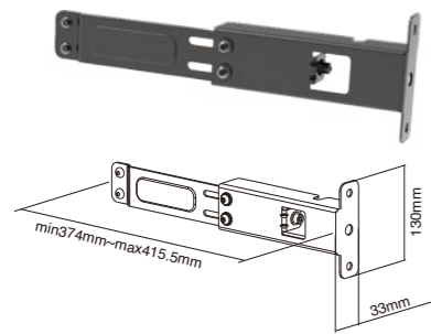
LVS02-B03 Permanent Fixed Base
