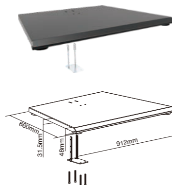
LVS02-B02 Pedestal Base
