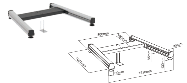
LVS02-B05 H Style Base with Leveling Feet
