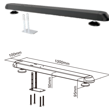
LVS02-B01 Floor Base with Leveling Feet
