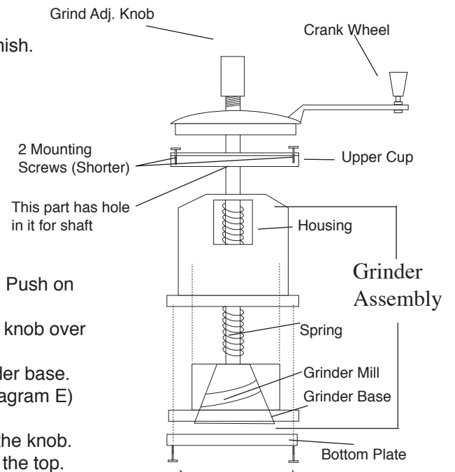
Diagram C Grind Assembly
