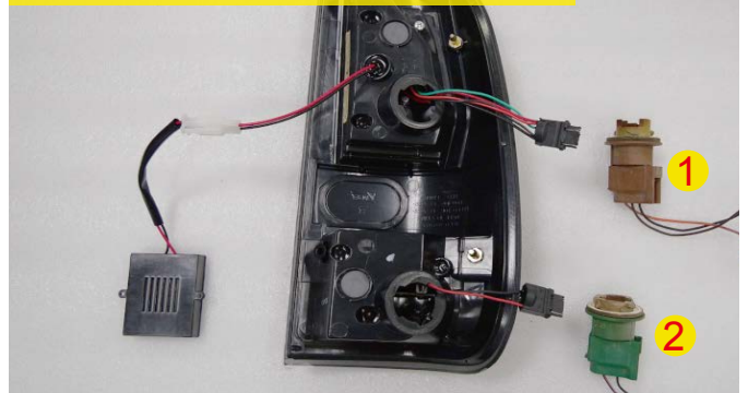
8. Reuse the factory bulb sockets.
