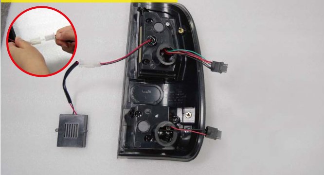
7. Connect the resistor.
