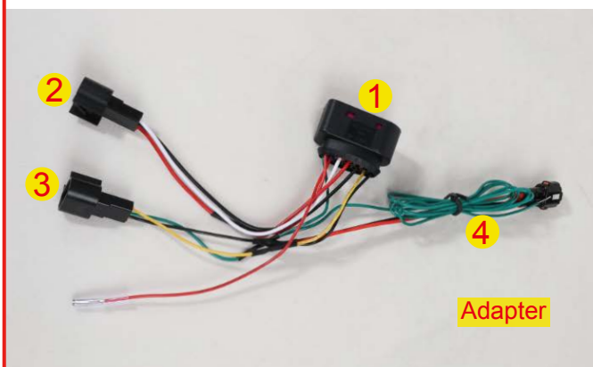
Plug the high beam and turn signal connectors.
