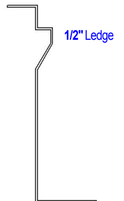
LEDGE PROFILE
