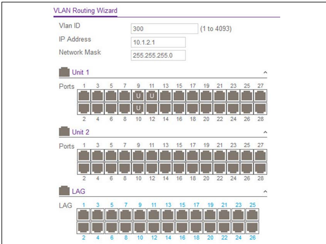
Figure 124. VLAN Routing Wizard
