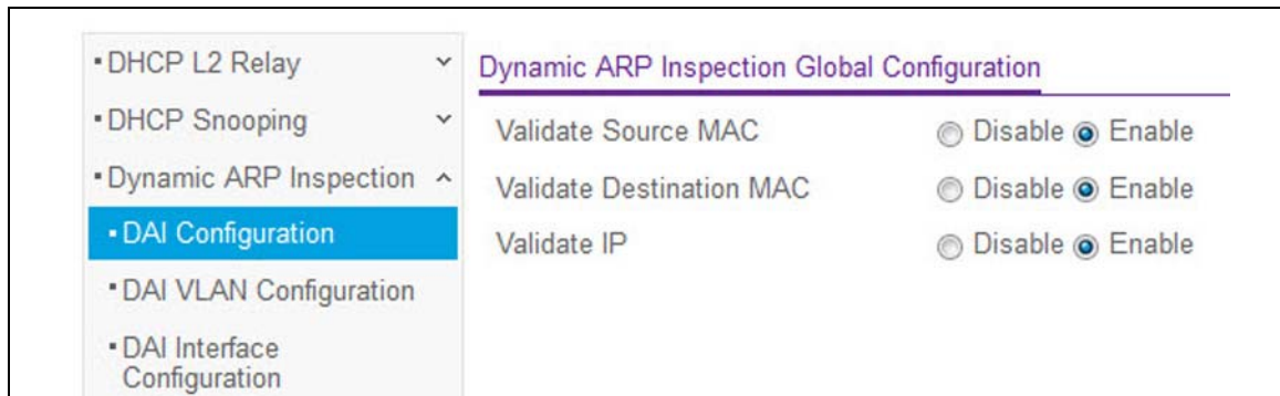
Figure 78. DAI Global Configuration
