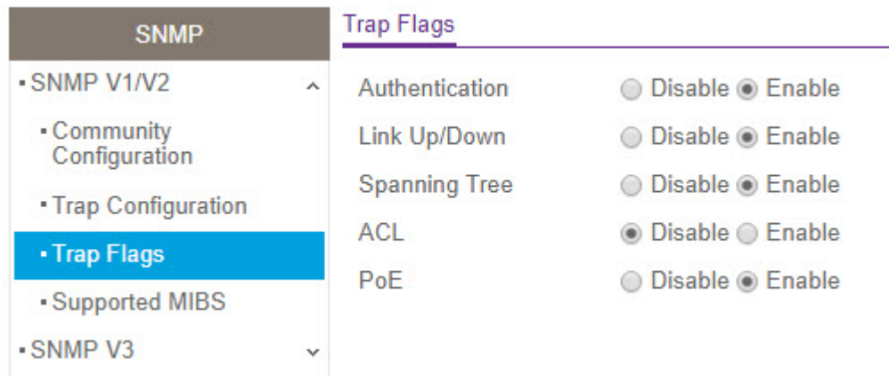
Figure 55. SNMP V1/V2 Trap Flags
