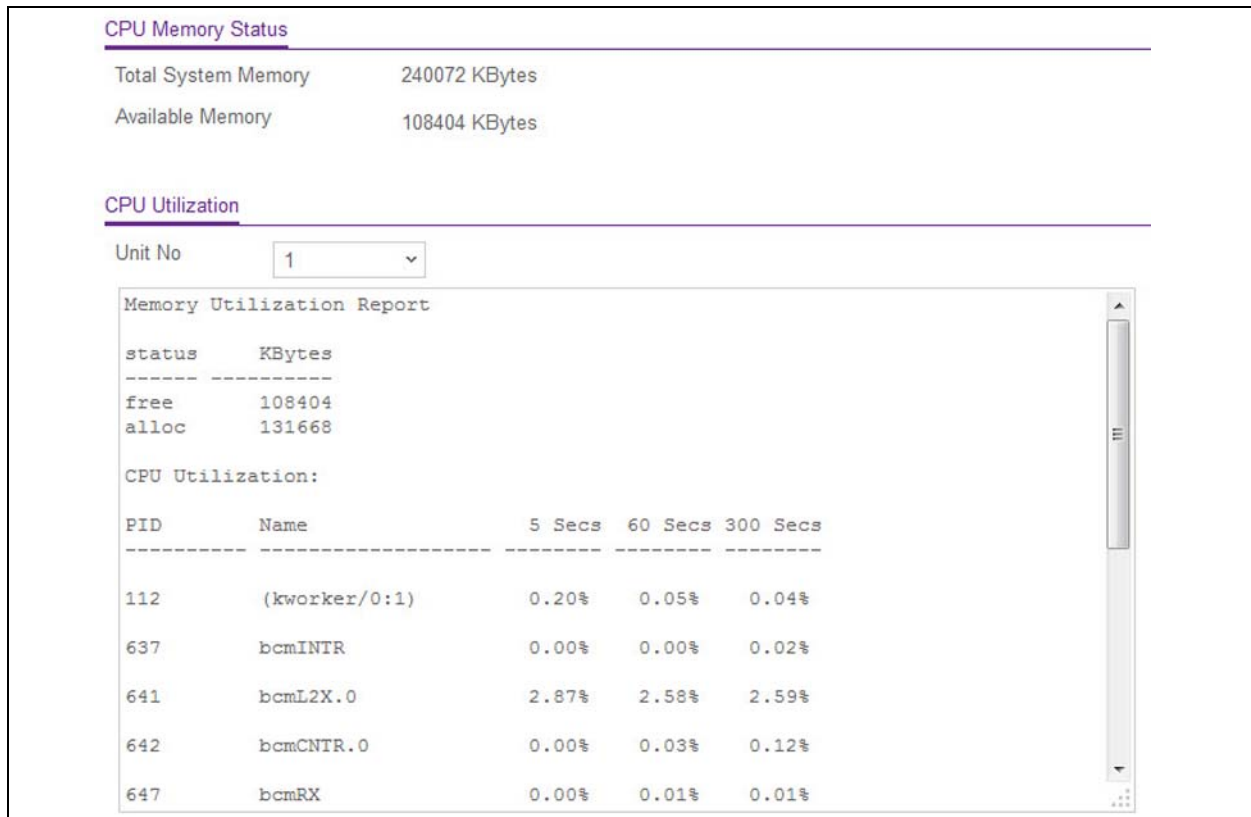
Figure 25. System CPU Status - Unit CPU Utilization
