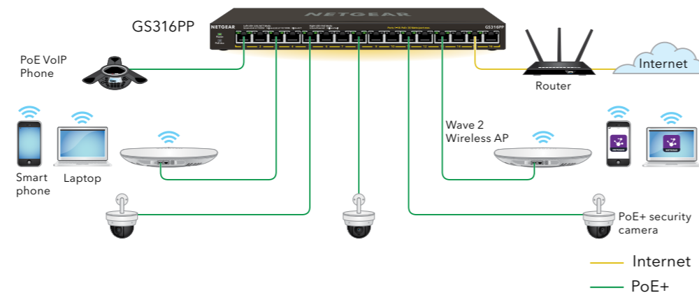
Sample connections
