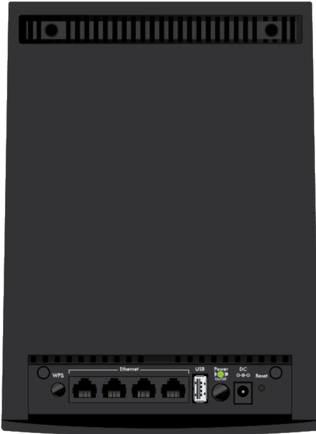
Figure 3. Back panel
