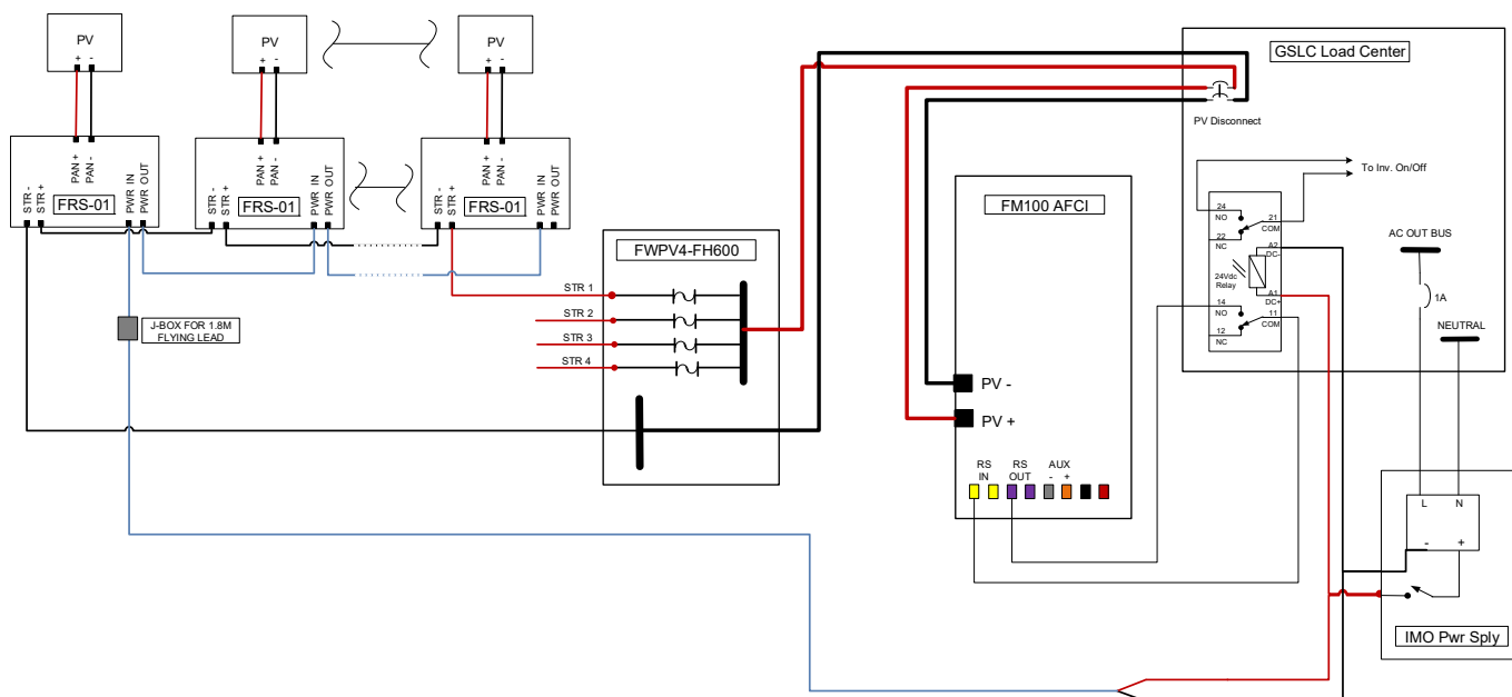
Figure 5 – Rapid Shutdown using IMO Fire Raptor MLPE devices and power supply with OutBack 24V DPDT relay
