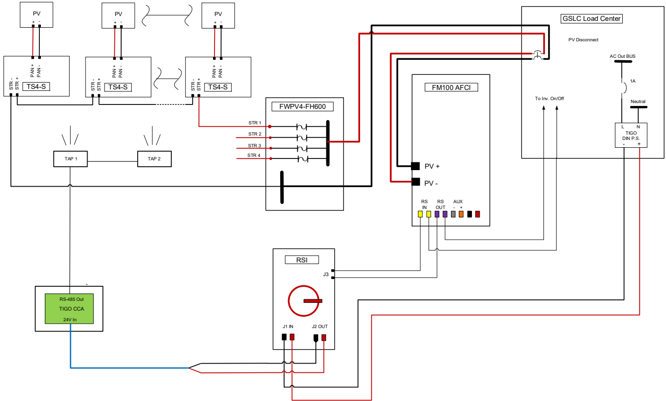
Figure 7 – 2017 Rapid Shutdown solution for Tigo MLPE devices and CCA Outdoor kit with OutBack RSI
