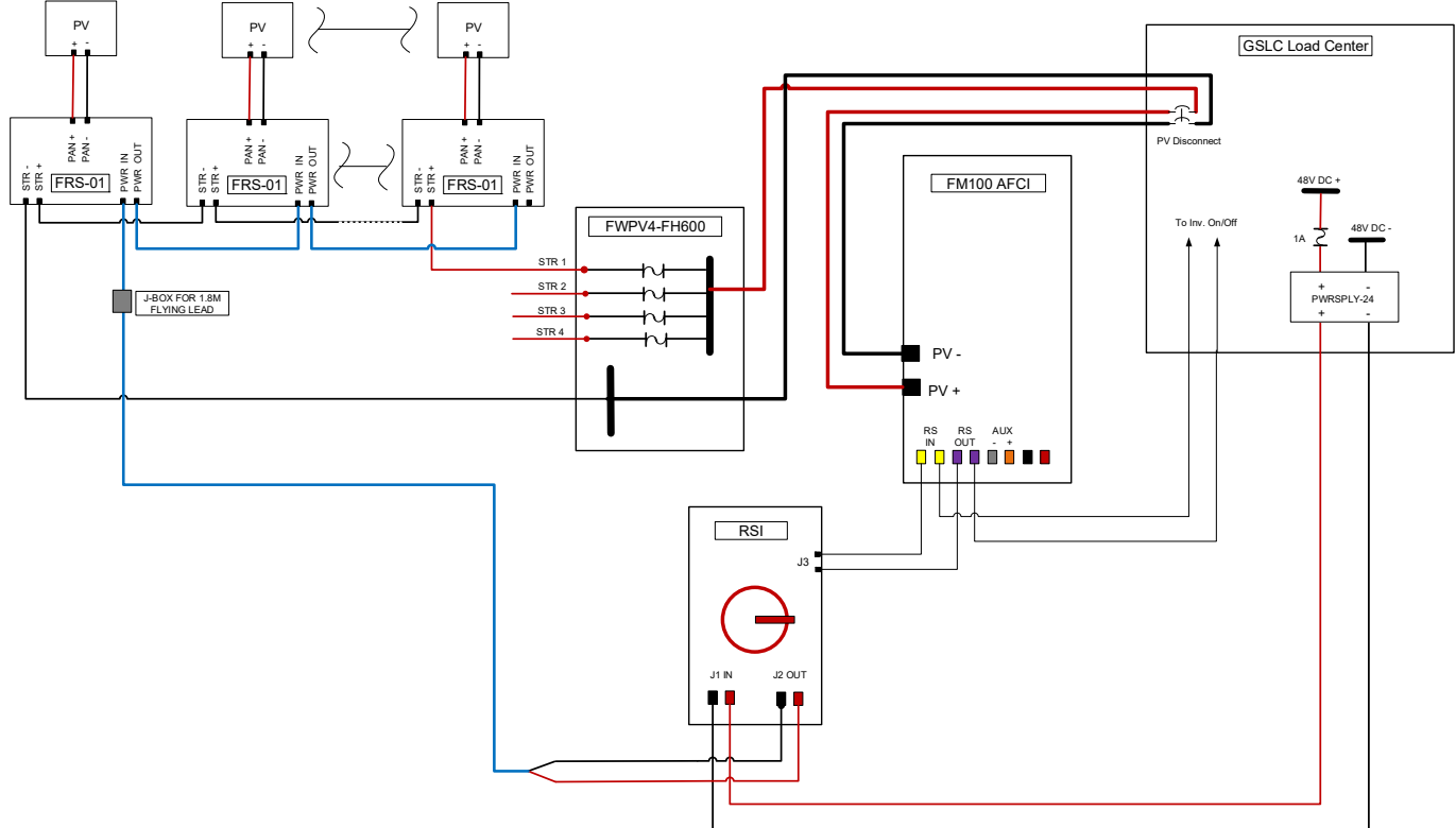
Figure 6 – Rapid Shutdown using the OutBack RSI and 24V power supply
