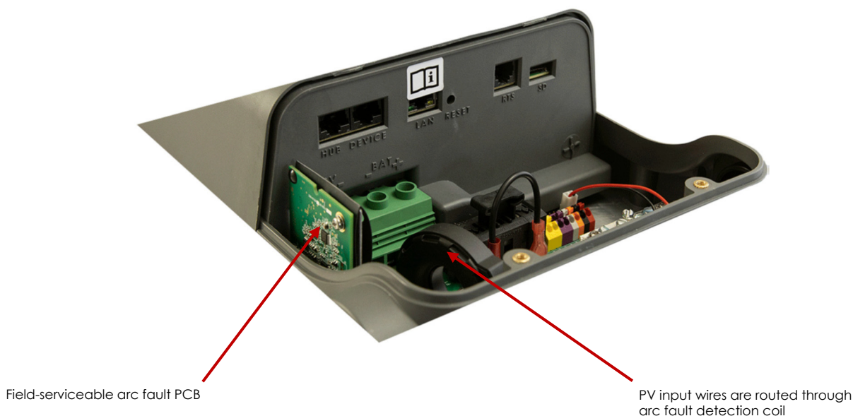
Figure 4 – Arc fault detection components
