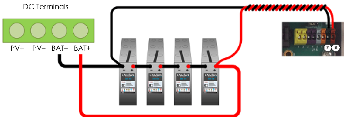
Figure 1 - Battery sense leads prevent unintended curtailment of parallel charge controllers
