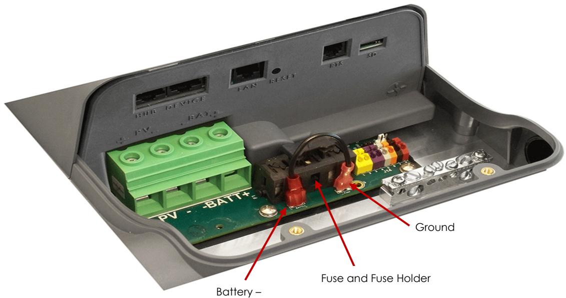
Figure 3 - Ground fault detection
