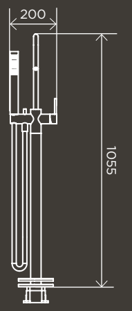
Round Freestanding Bath Spout MB06
