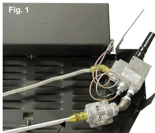
Gas Supply
