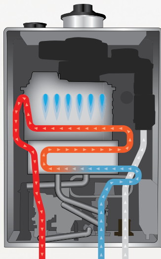
HOT WATER OUTLET COLD WATER INLET GAS INTAKE
