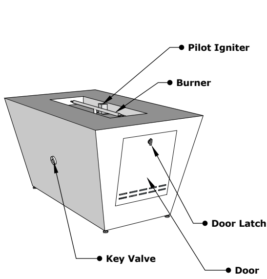
ISOMETRIC VIEW
