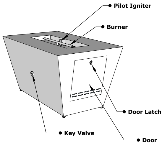
ISOMETRIC VIEW
