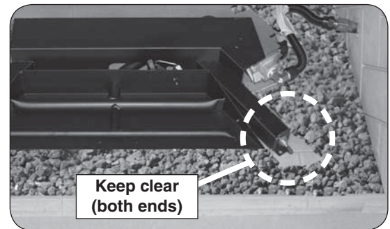
Fig. 18-2 Proper lava media placement
