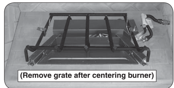
Fig. 17-3 Position grate
