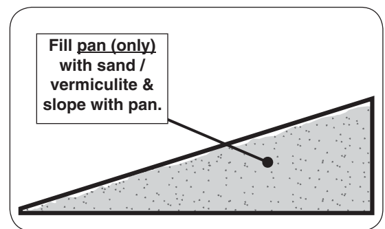
Fig. 18-4 Sand/vermiculite detail
