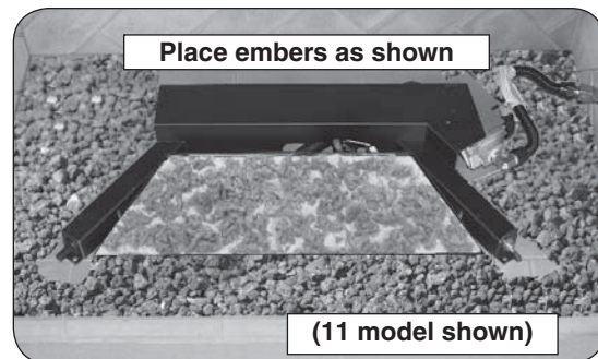
Fig. 19-1 Place glowing embers
