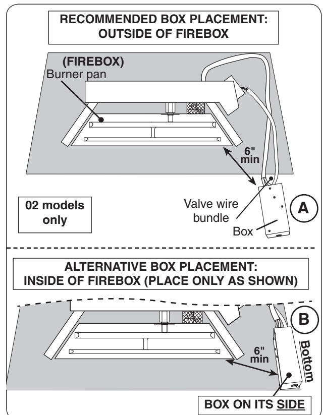
Fig. 16-3 Switch box placement (if applicable)
