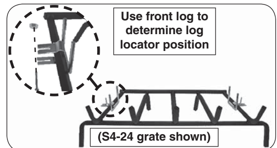
Fig. 17-2 Attach log locators to grate
