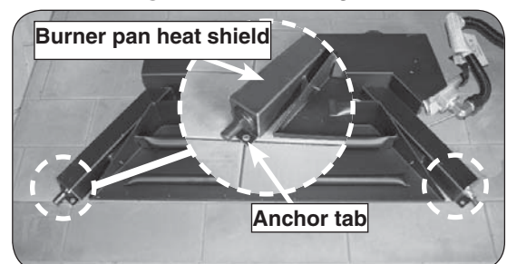
Fig. 17-4 Secure burner to floor
