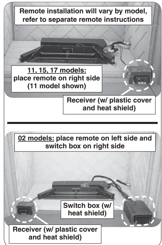
Fig. 17-1 Install remote receiver and heat shield(s) (as applicable)
