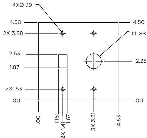
E-STOP/SWITCH CONTROL PANEL COMBO
