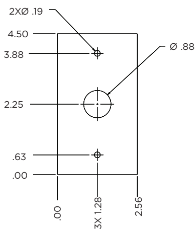
E-STOP CONTROL PANEL
