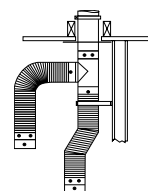
COMBINED VENT TO CEILING
