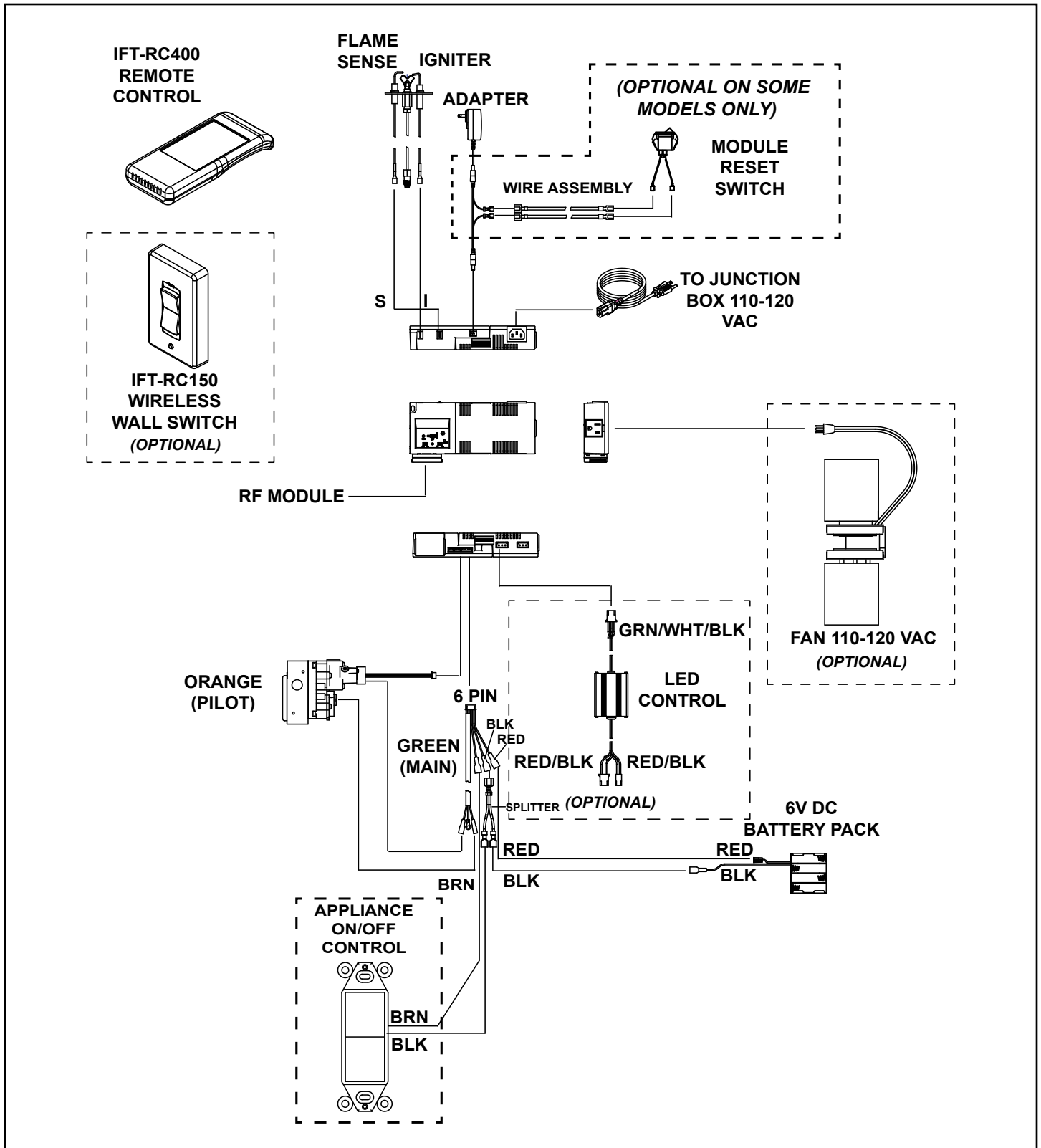
Figure 6. Wiring Diagram without Power Vent
