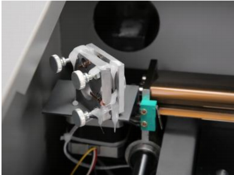
Figure 5-5 Alignment set screws for the second Mirror
