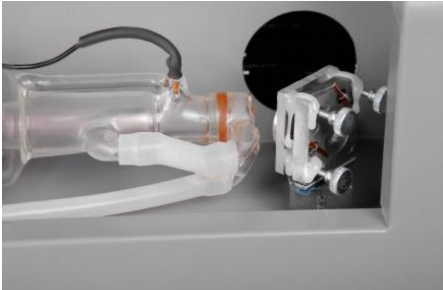
Fig. 5-2 Adjustment set screws Behind the First Mirror
