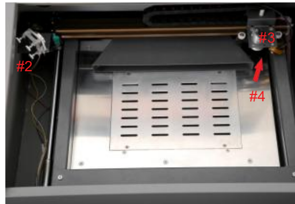
Fig. 1-2 Mirrors #2-3 & Focus Lens
