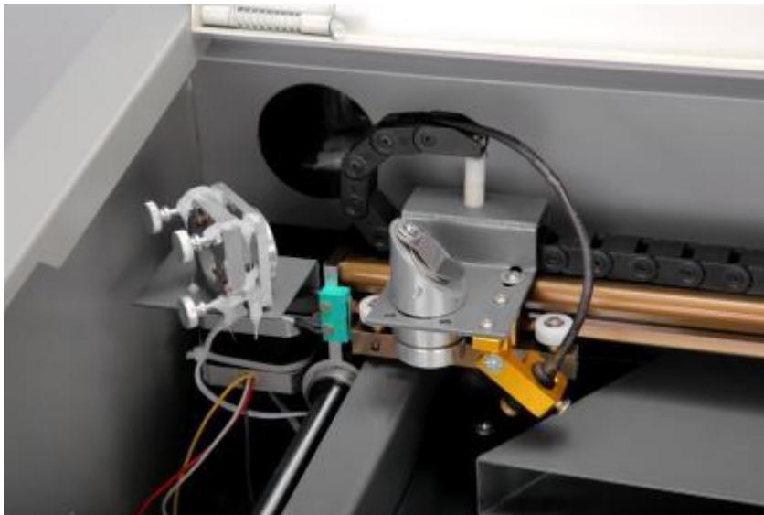
Fig. 5-1 The second Mirror in Position A
