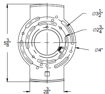
Mounting Back Plate Dimensions PD-48932&PD-48948
