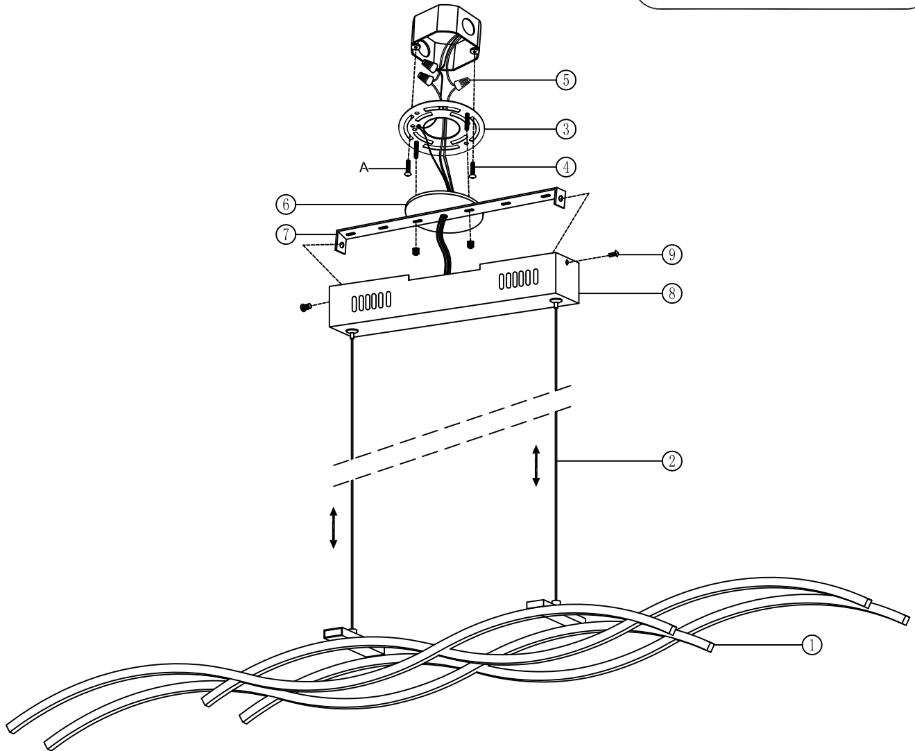
Wire connection
