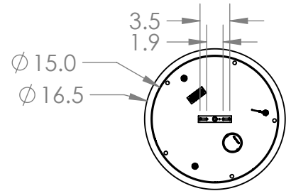
Mounting Detail MOUNTS TO BUILDING STRUCTURE
