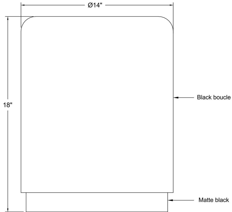
FRONT VIEW
