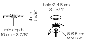
recessed canopy
