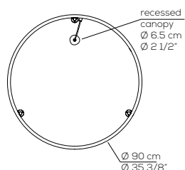
recessed canopy
