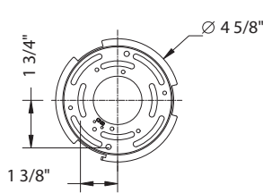
CEILING PLATE
