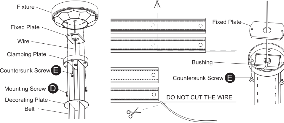
Fig. 4 Wire Diagram
