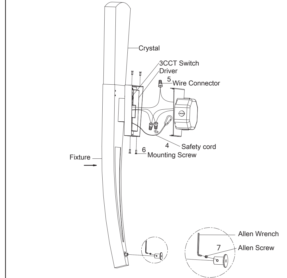
Fig.3 Driver Wires
