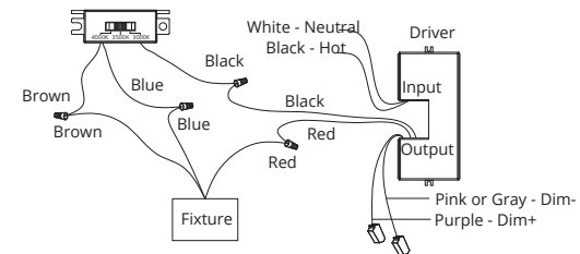
Fig.3 Driver Wires
