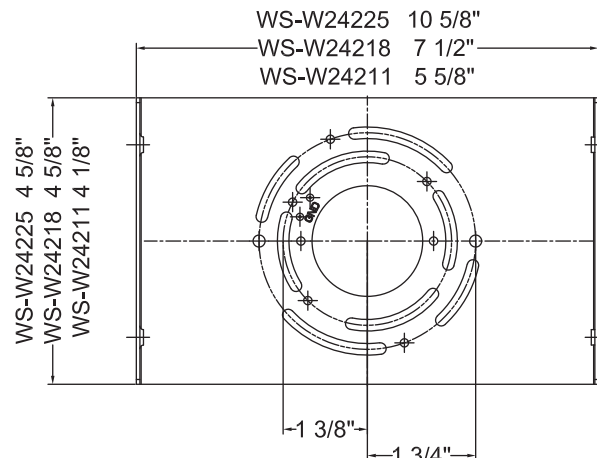
Mounting Back Plate
