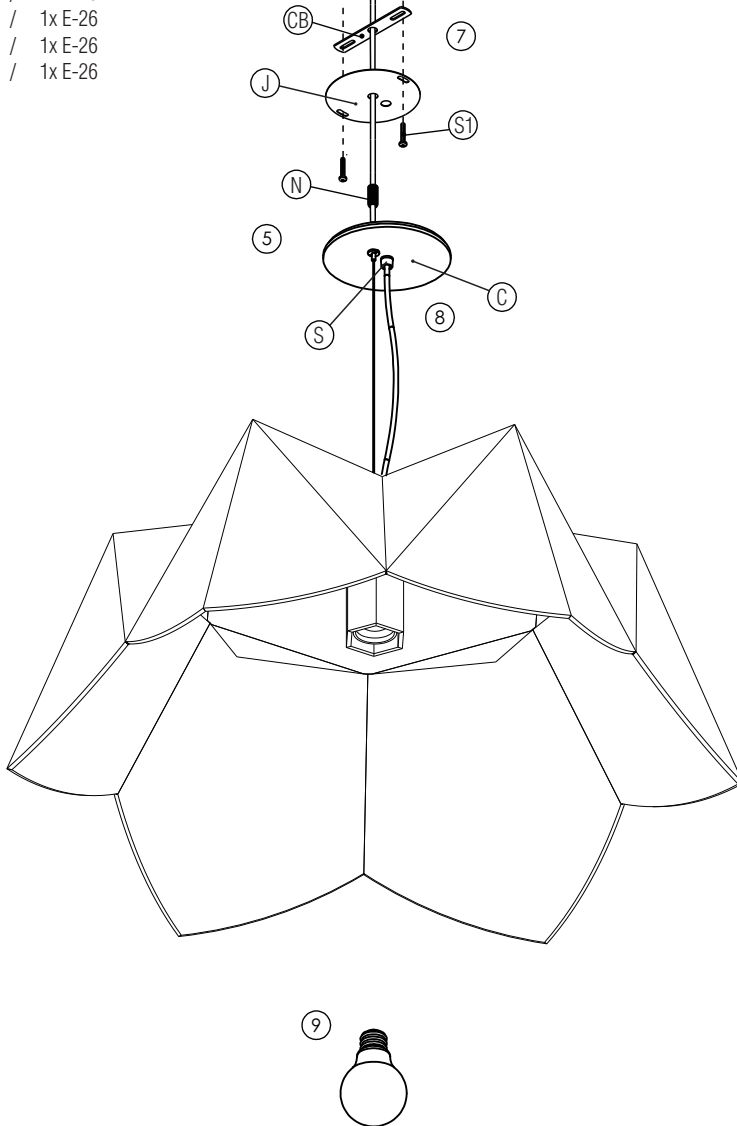
PROVIDED SCREWS
