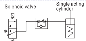
Meter-in speed controller
