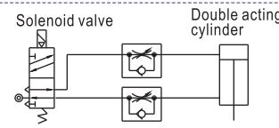
Meter-out speed controller
