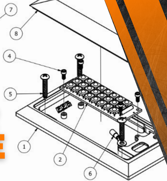
Truck Dome Light
