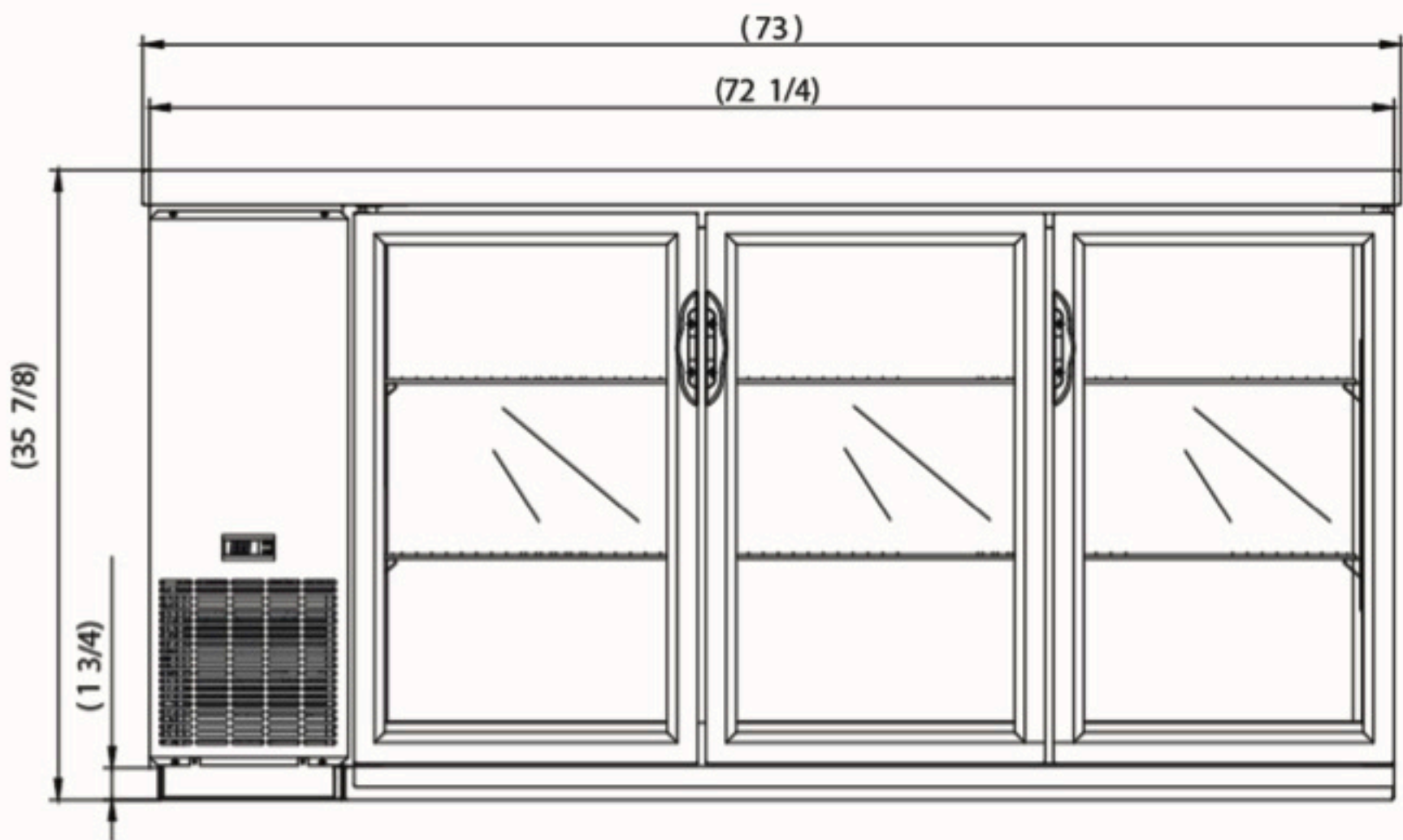
Front View
