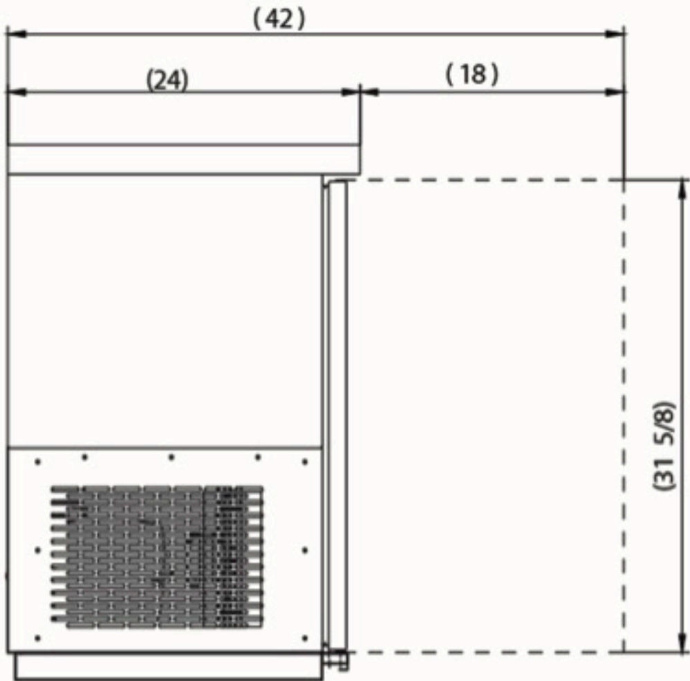
Side View
