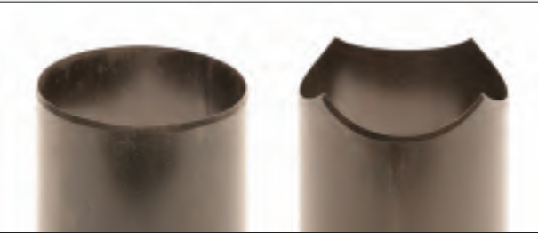
Outside sharpened: push up native soil
