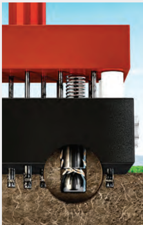
Seed filled spikes extended.
