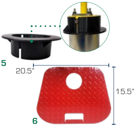
5. Hole Cutter Flanged Stop [No. 217]
