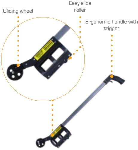
Marking Wand [No. 268]
