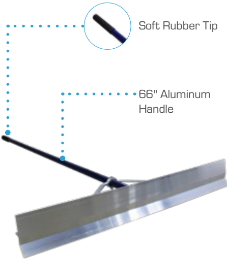
Aluminum Plug Pusher [No. 131]
