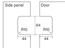
Glass cutout
