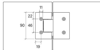
Glass cutout
