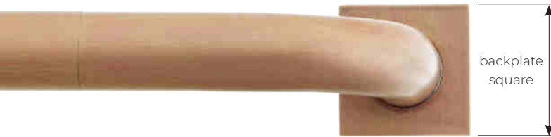
new French Return with Square Mount Plate (Includes Pole Splice; Metal Pole sold separately) PO138MEFRS 3 1/2" return, 5 1/2" L, 2 7/16" backplate W, 3/8" plate thickness Metal, Blush
