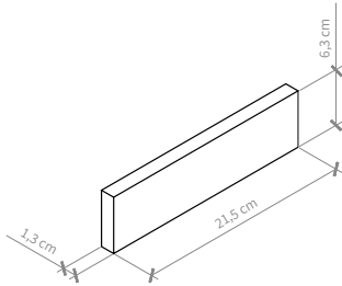
VICTORIAN BRICK
