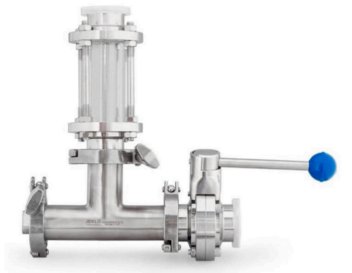
Kit for wort oxygenation, prior to entering the fermenter.
