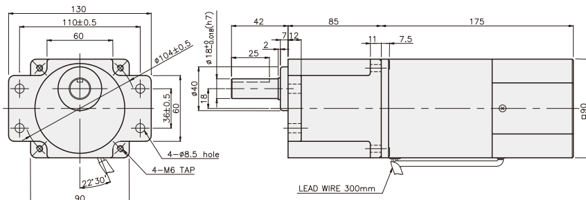
K9RP90F□-SP + K9P□BUF
