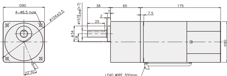
K9RP90F□-SP + K9P□BF
