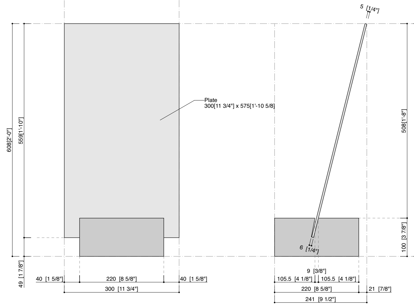
Front view
