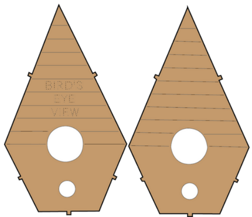
FRONT + BACK WALLS
