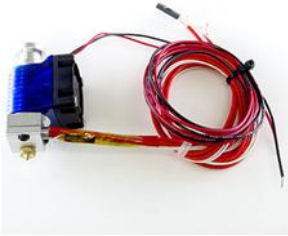
Hotend (Assembled)
