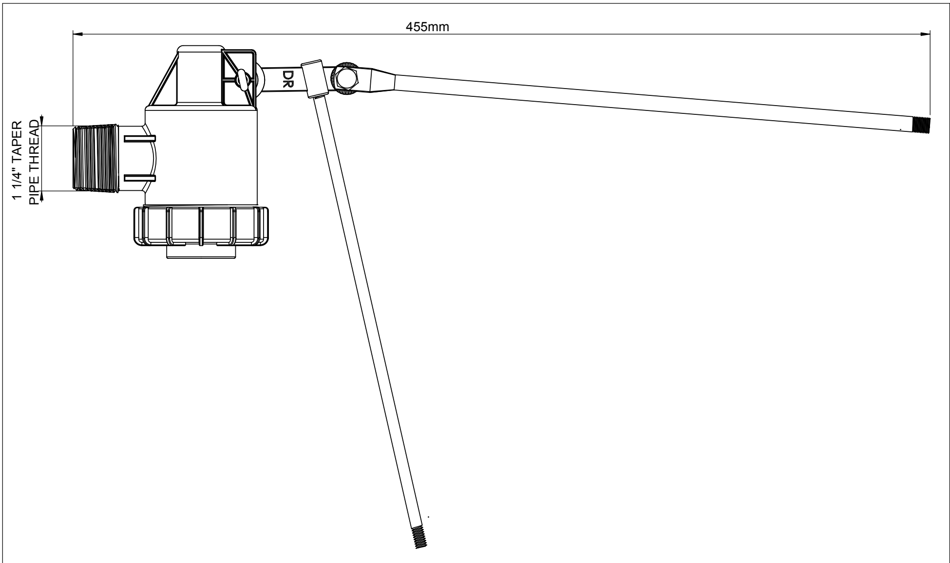
Dual level reservoir valve RES DL-32
