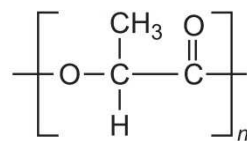
poly(2-hydroxypropanoic acid) poly(lactic acid), PLA
