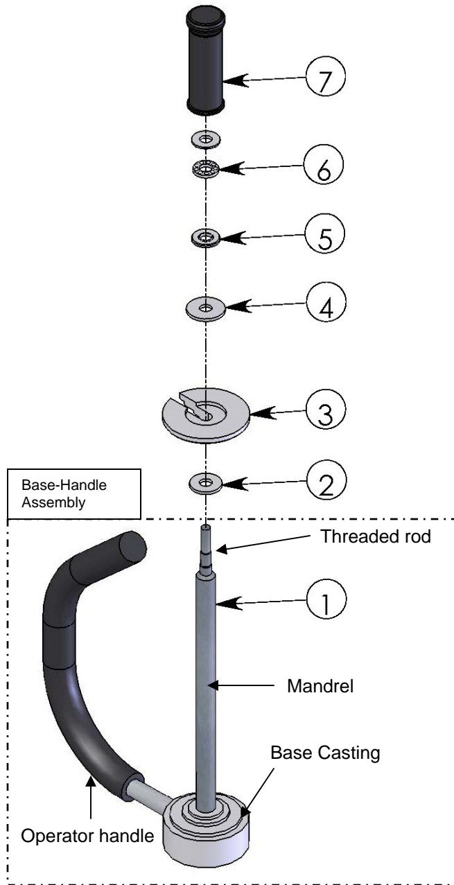
FIG. 1: Exploded Parts Diagram
