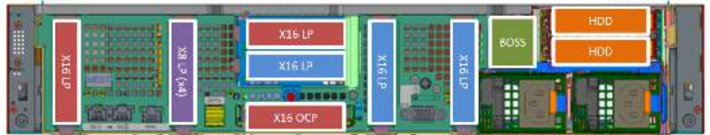
Figure 10. Rear view of the system
