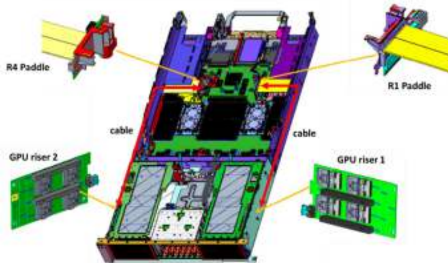
Figure 19. GPU Riser ½ connection with R1/R4 paddle by cables
