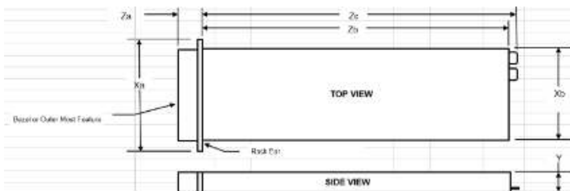
Figure 27. Chassis dimensions
