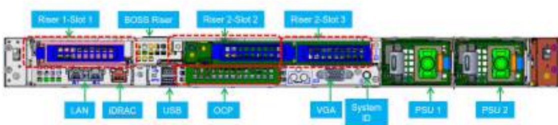
Figure 8. Rear view of the system Riser 1, Riser 2a
