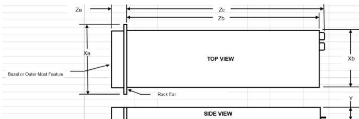
Figure 32. Chassis dimensions
