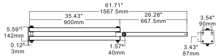
60" Bracket C3
