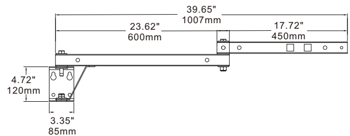
40" Bracket A2, Built-in receptacle
