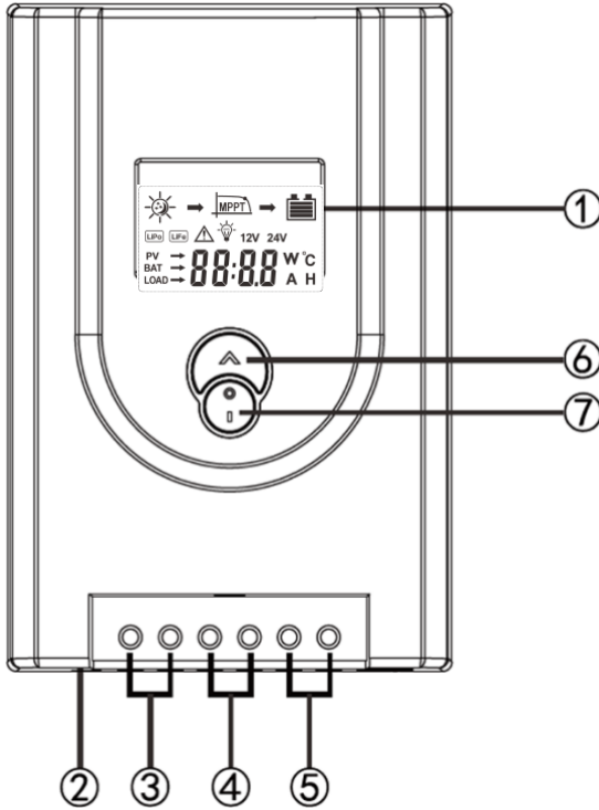
Figure 1 Solar Controller Features
