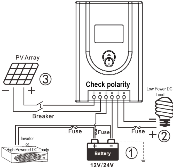
Figure 3 Connection Diagram
