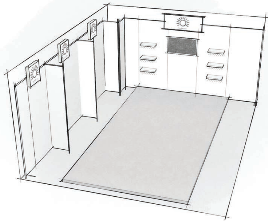
Showroom Layout 16' x 20' includes structure, TV mount, shelving, overhead lightboxes and graphics.
